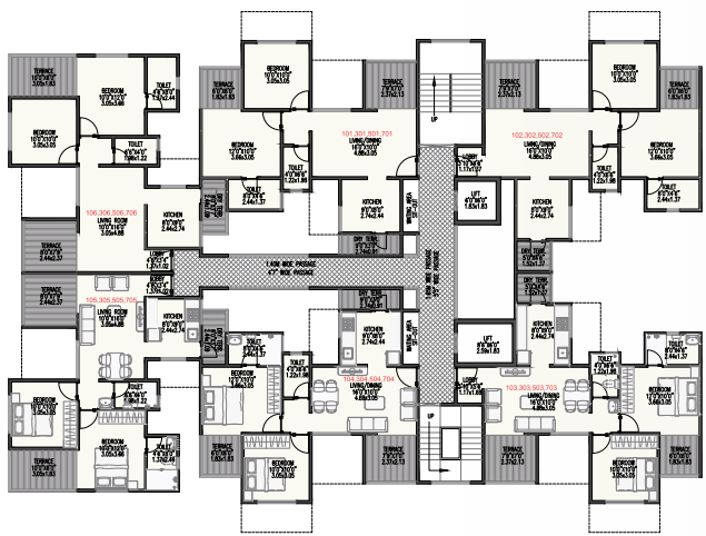
C WING TYPICAL ODD FLOOR PLAN 1st, 3rd, 5th, & 7th FLOOR
