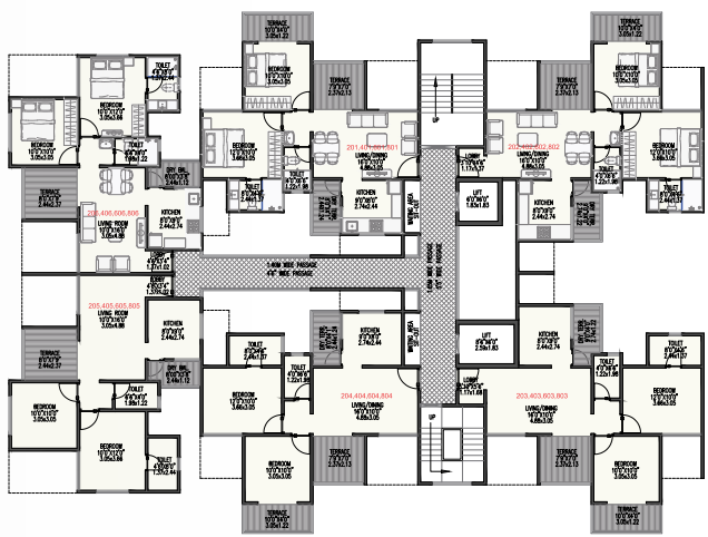
C WING TYPICAL EVEN FLOOR PLAN 2nd, 4th, 6th, & 8th FLOOR
